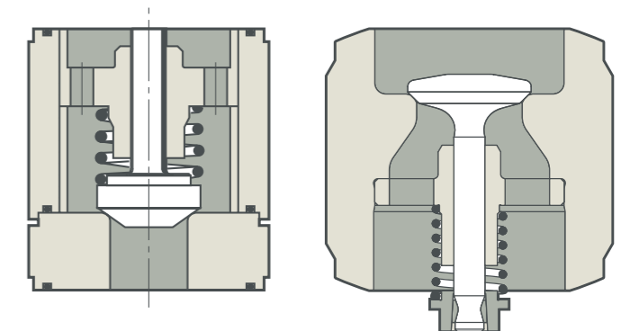
Cone valve
