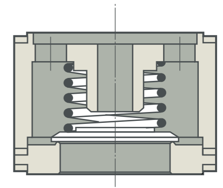
Disc valve
