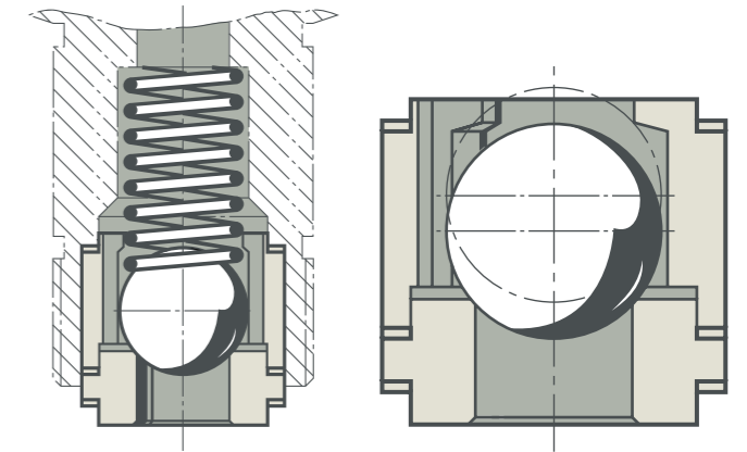
Ball valve
